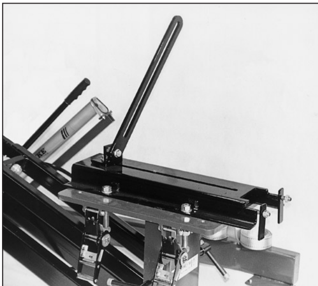
The rear-axle-gear holder is mounted on the top of the gear-box lifting device plate.
