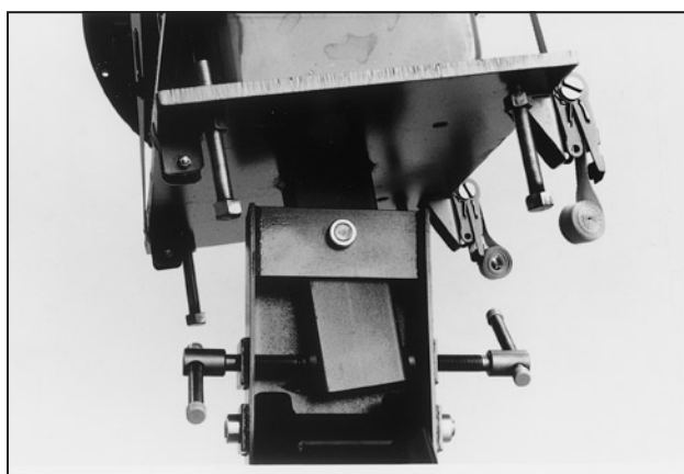
Stepless tipping of the fixing device plate side-wise by 2 pcs of attachment screws.
